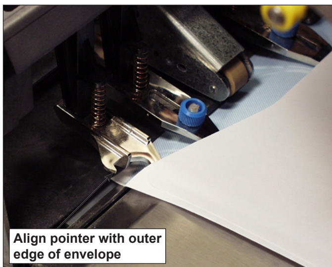
Figure 3.9.3: Aligning the Outer Envelope Opener
