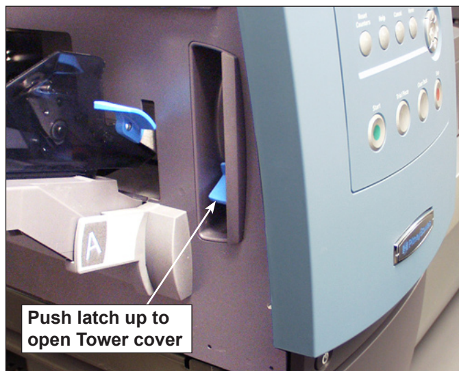
Figure 2.2.1: Latch Opens Feeder Tower.
